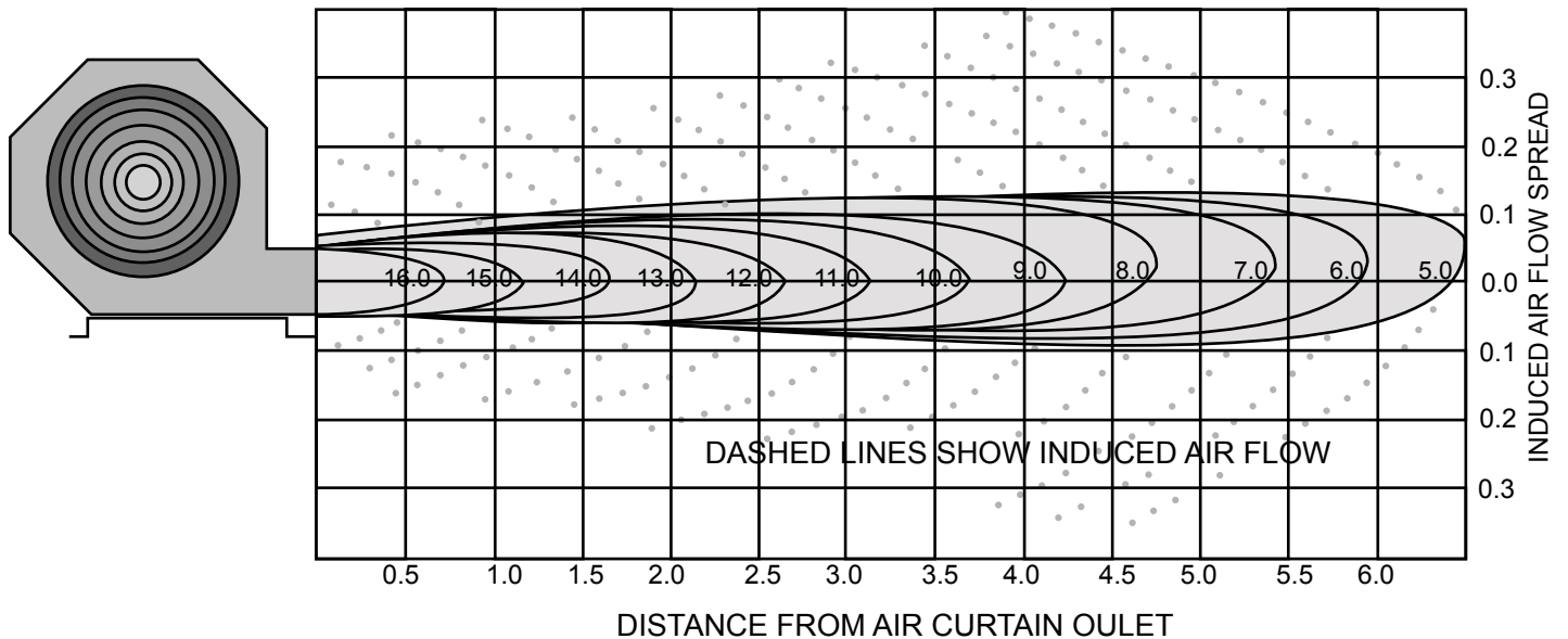
AIR CURTAIN VELOCITY CONTOURS (M/sec)
